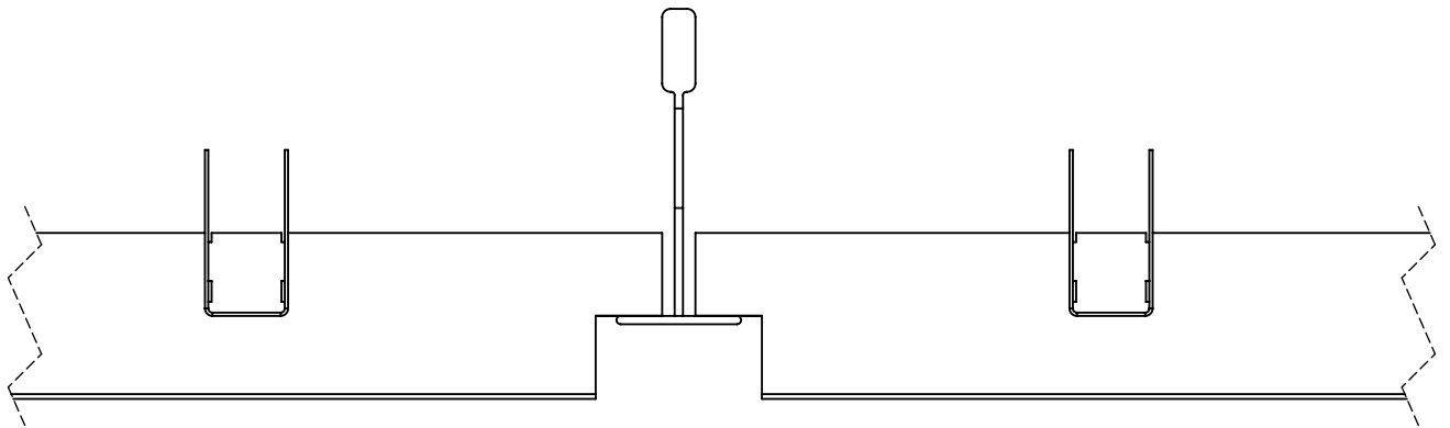
DeltaCell-Line regular Lay-in system
