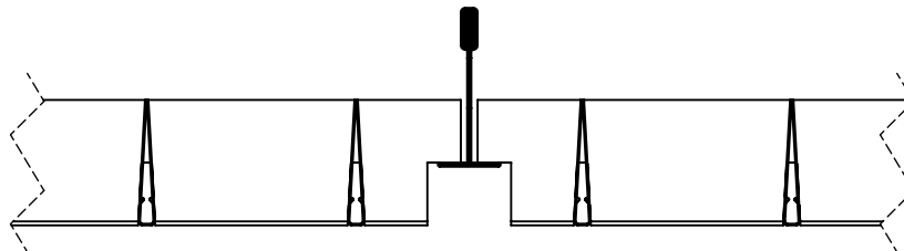
DeltaCell tegular Lay-in system
